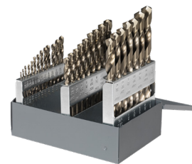
Order #C21121 29 pc. Jobber Drills 135° Split Point, Straw 1/16" - 1/2" x 1/64" $147.00
